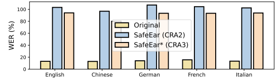
(b) WER comparison on the CVoiceFake dataset
