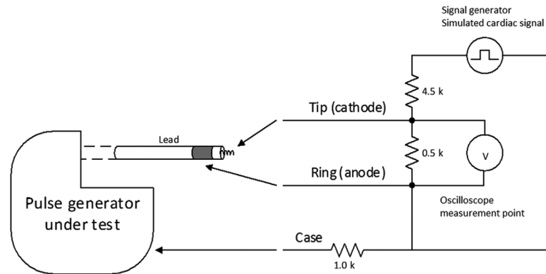
FIGURE 1 St. Jude Assurity pacemaker pacing and measurement setup
